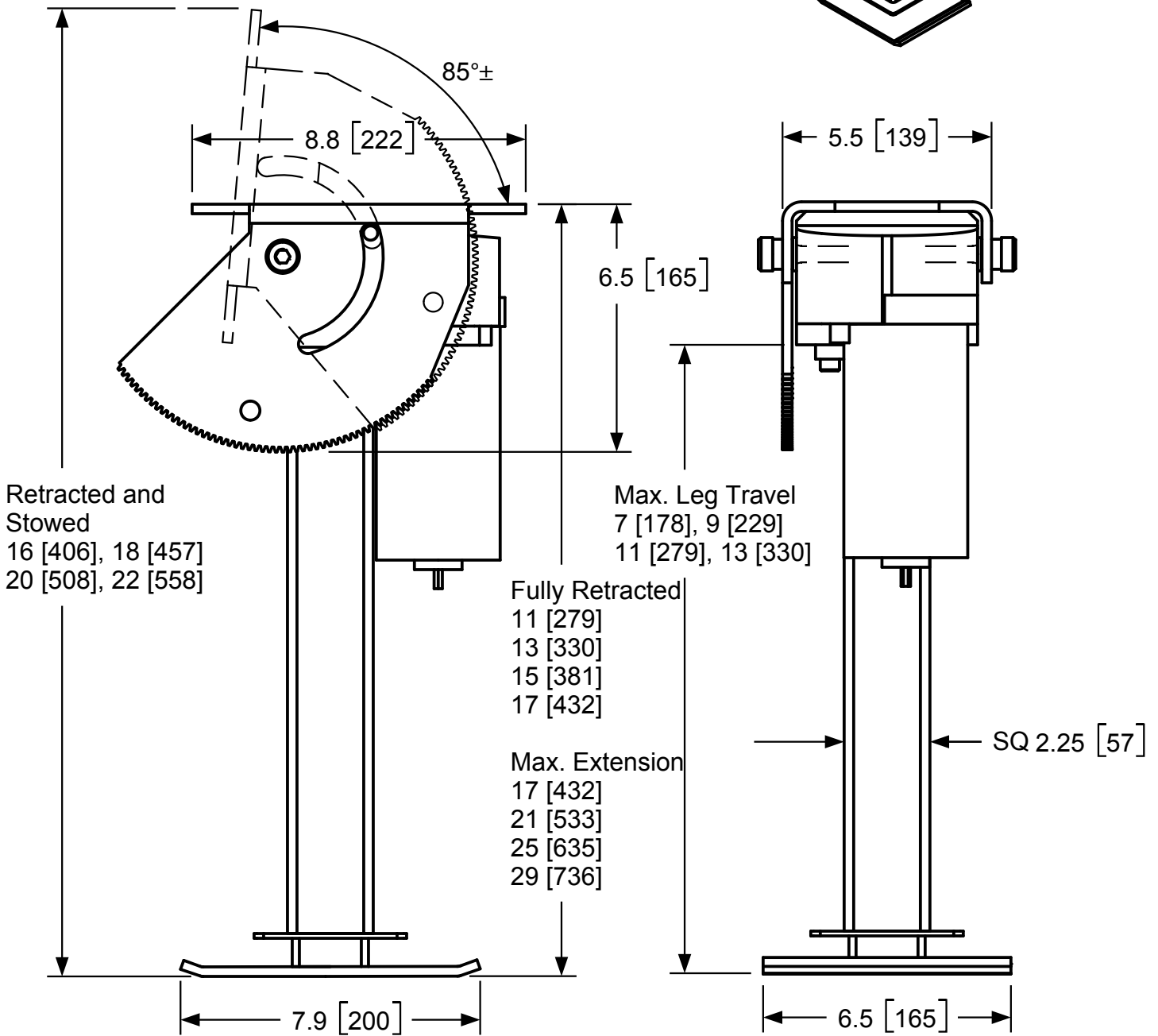
FOLDING LEVELING JACK INCHES [MILLIMETERS]
